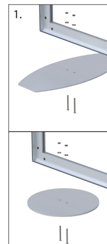
XSMA/XSMB with Base Plates
